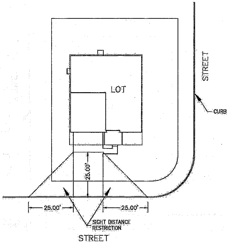
TYPICAL SIGHT DISTANCE RESTRICTION AT DRIVEWAY APPROACHES
